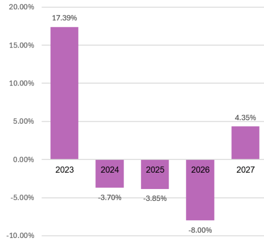
ERP
