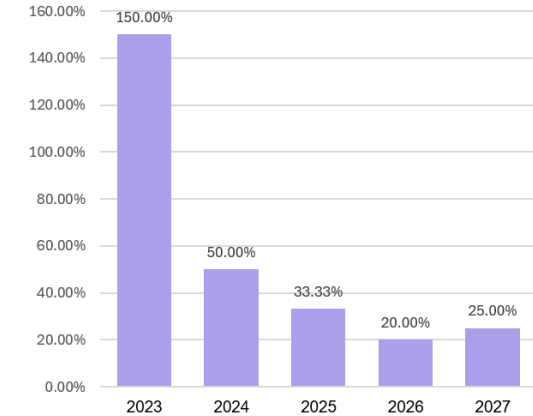
Military Software
